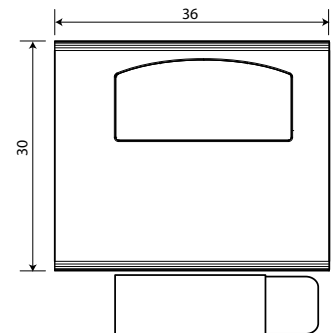
SHL-363030-RK/LC Single table with casters
