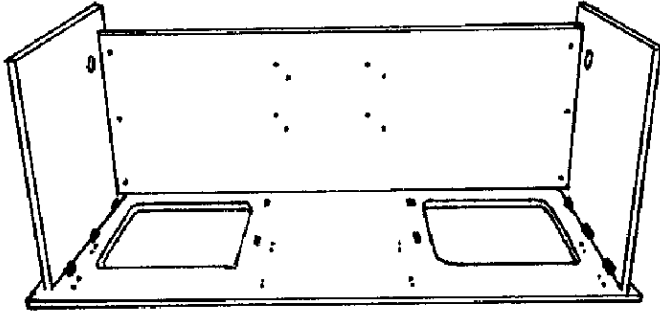
Figure 7 Smartdesks with Side & Back Panels Assembled
