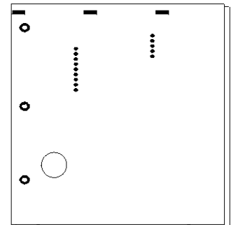
Right End Panel (1 ea.)
